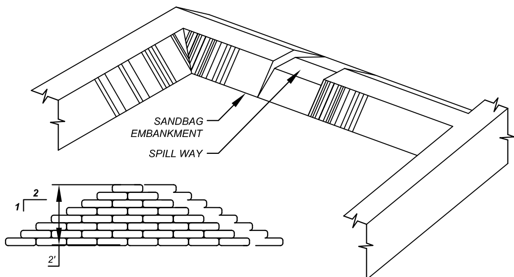
TYPICAL SANDBAG STACK FOR SPILLWAY APPLICATION
