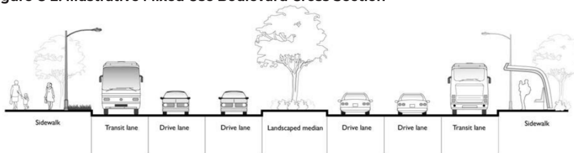
Figure C-2: Illustrative Mixed Use Boulevard Cross Section
